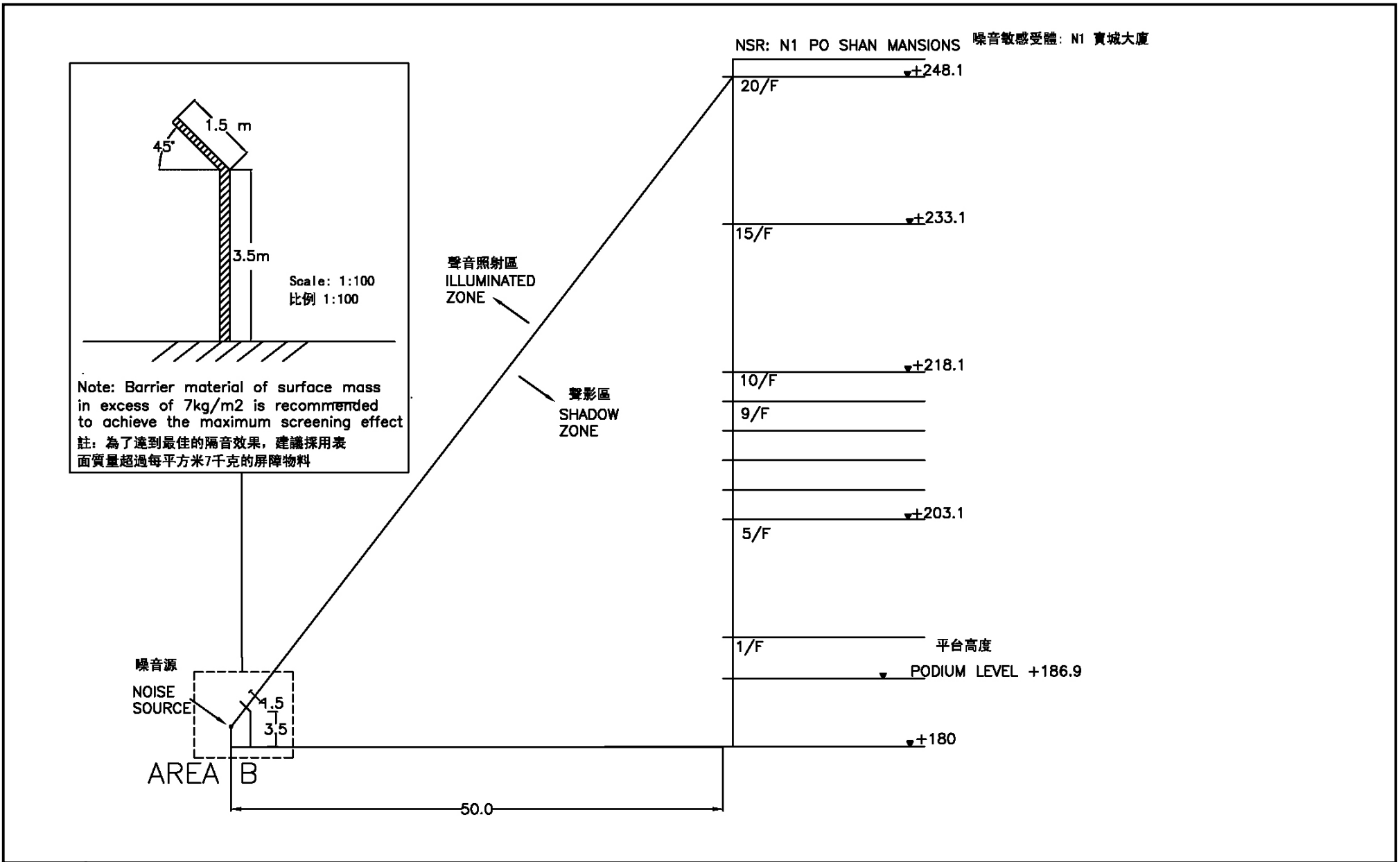
Figure 8 - 2 : Typical Section of Movable Noise Barrier (for part II of the project) 圖 8 - 2 : 流動隔音屏障的切面圖 (適用於工程項目第 II 部份)
